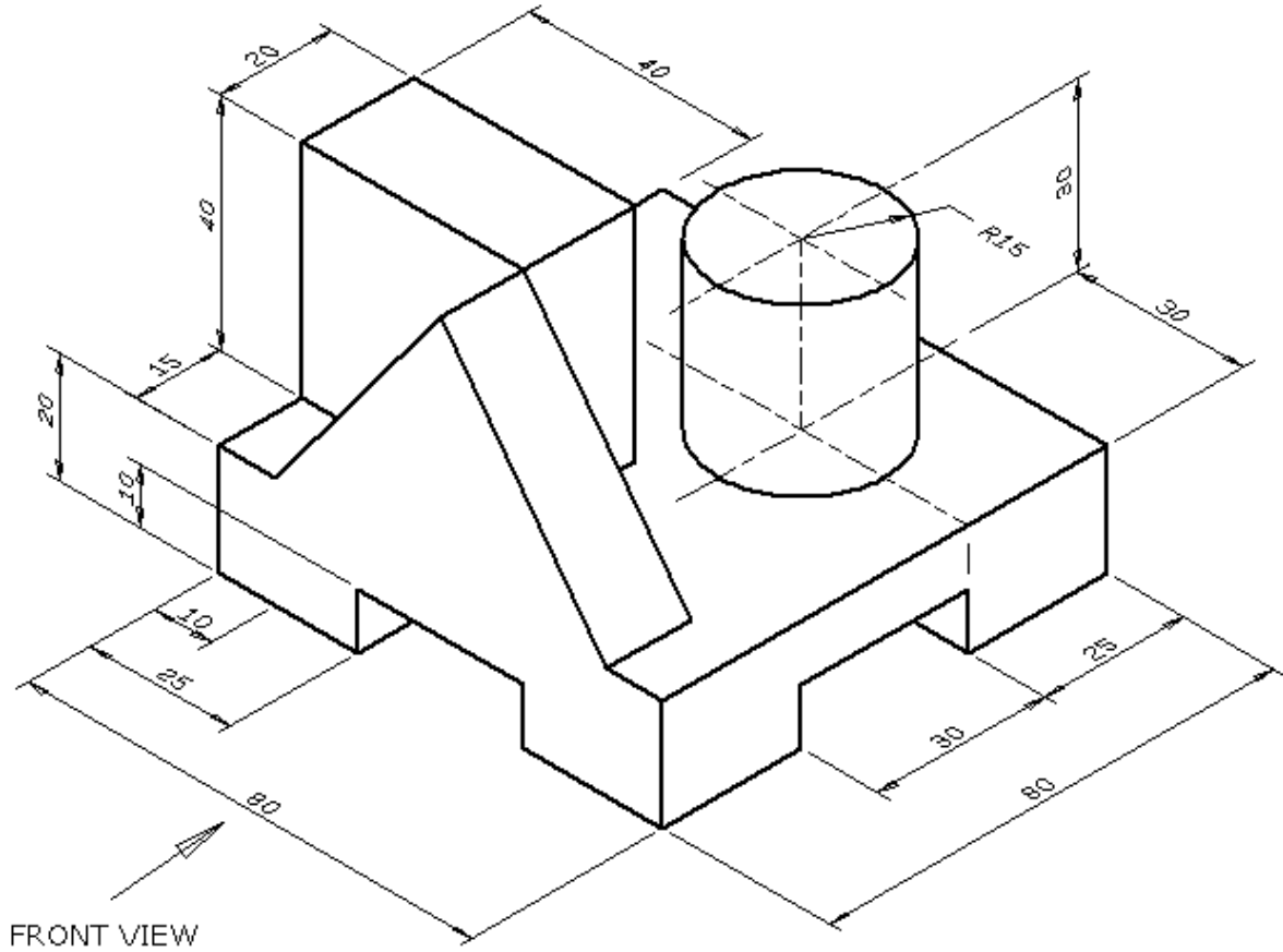
SHAFT BRACKET
