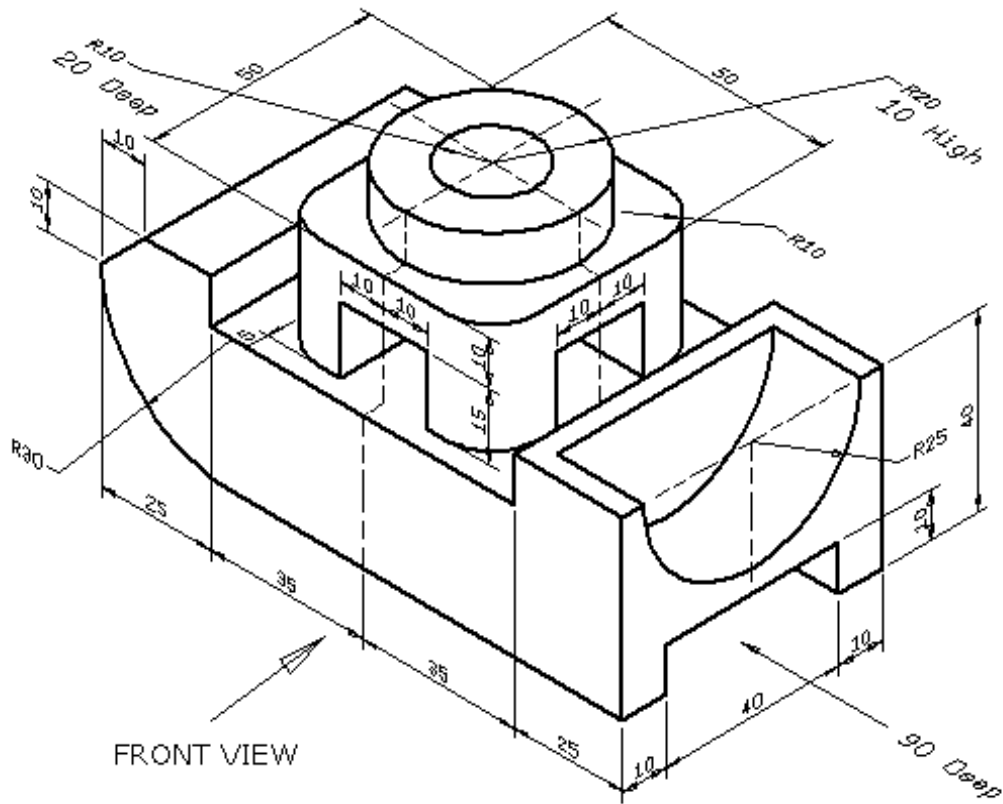
SHAFT BRACKET
